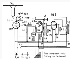
2m-Transveiver Willy Fischer, DL1AG
