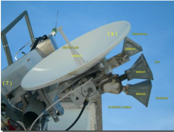
OE7XVR Sendeantennen
