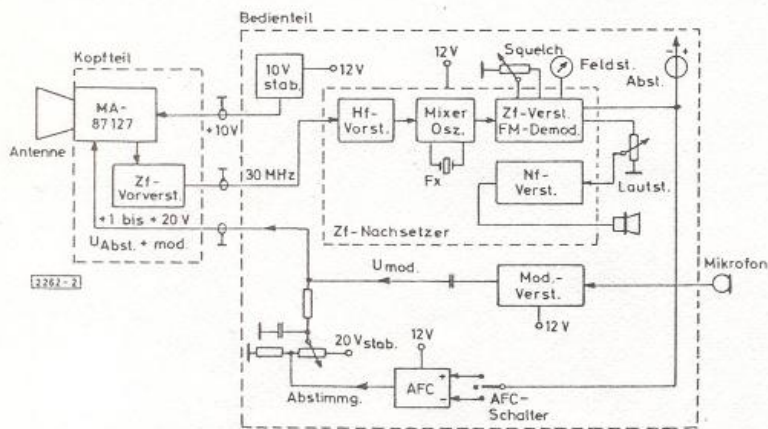
Abb. 2. 10-GHz-Transceiver, Blockschaltbild
