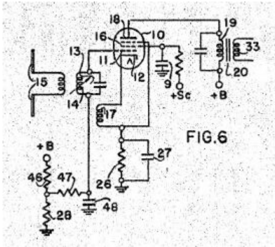
Superregenerative Receiver for 2 Meters
