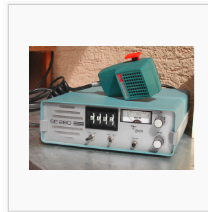
Mobil-FM-Transceiver SE 280, 144-146 MHz in 80 Kanälen
