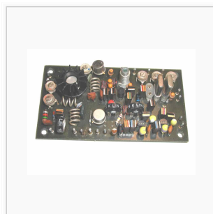
Hael SB-II Portable 2m AM/FM Sender
